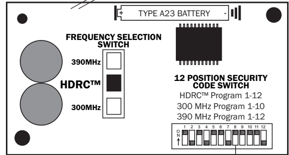
FIGURE 1 Transmitter Circuit Board
