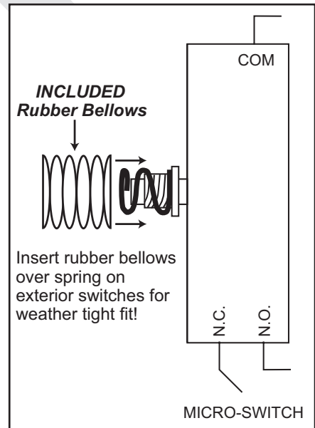
BELLOWS DIAGRAM
